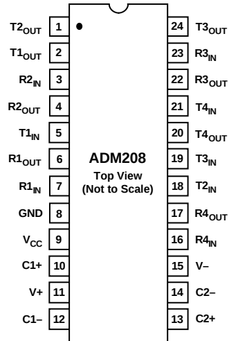
Figure 7. ADM208 DIP/SOIC/SSOP Pin Configuration
